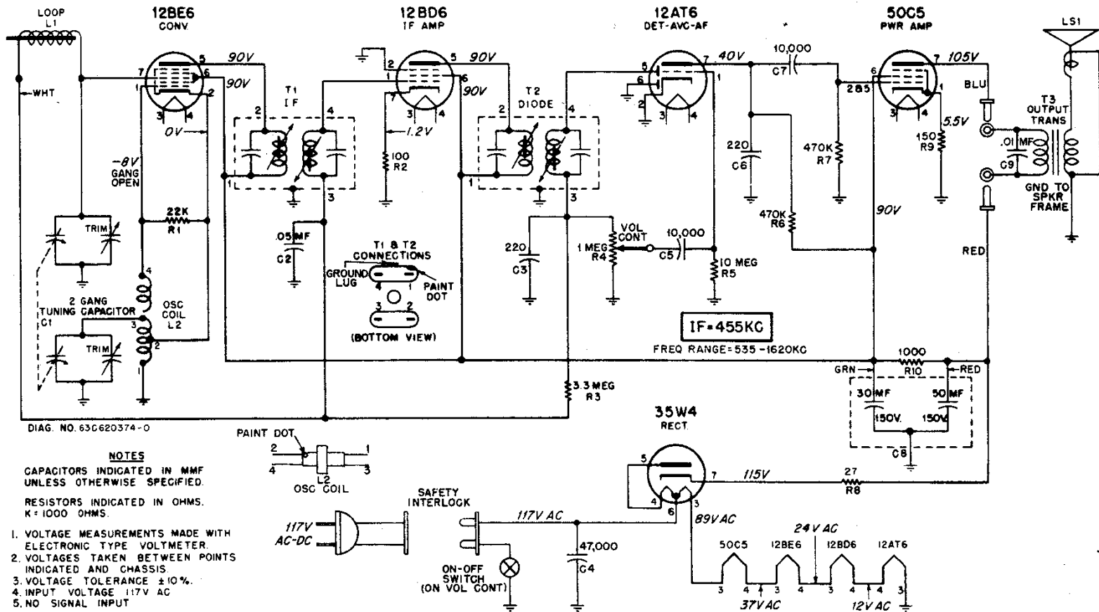
FIGURE 7. SCHEMATIC DIAGRAM
